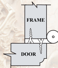
OPTION 3 OVERLAY
