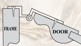
HINGE 1 1/4" OVERLAY
