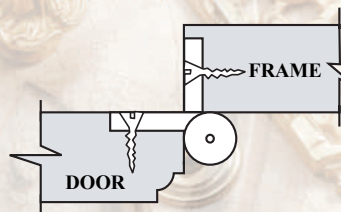
OPTION 2 OVERLAY
