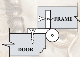
OPTION 1 OVERLAY
