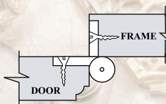
OPTION 2 OVERLAY
