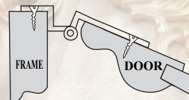
1/4" OVERLAY
