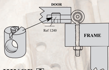
HINGE #3 11.1240 SUPPLIED WITH HINGE #3
